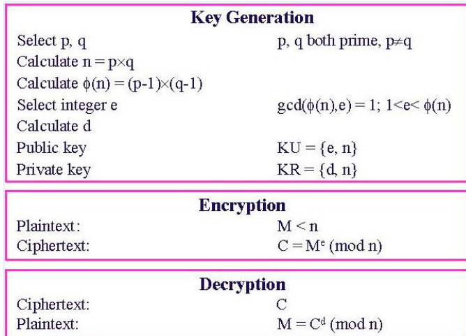
Figure 1. RSA Algorithm
