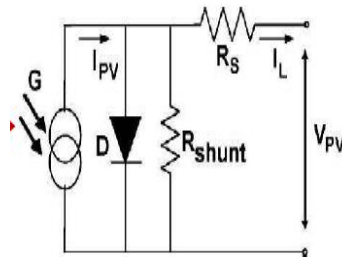
Fig 3. Circuit diagram representation of Solar cell
