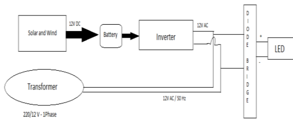
Fig 8. Proposed Block diagram of Hybrid Power System.
