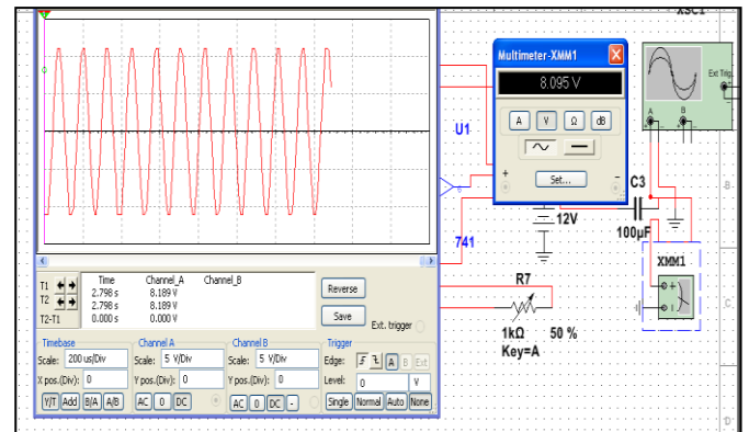
Fig 9. Output waveform of Hybrid Power System model
