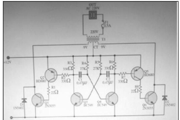
Fig 6. Circuit diagram of Inverter
