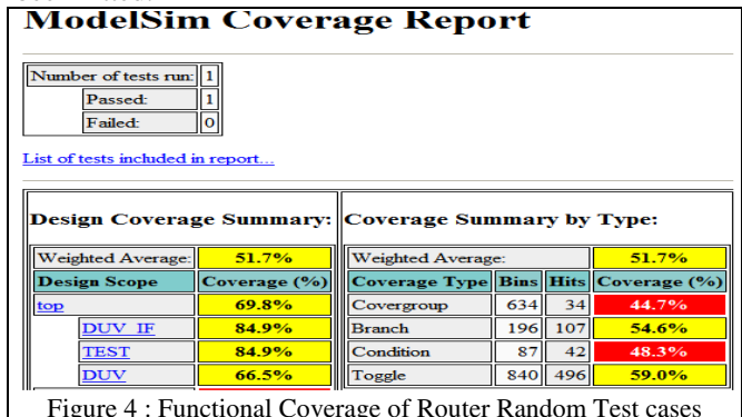
Figure 4 : Functional Coverage of Router Random Test cases
