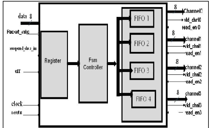
Figure2: Internal Structure of Protocol
