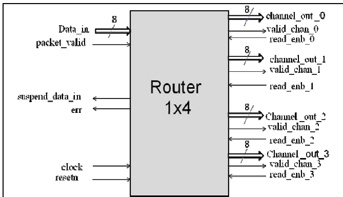
Figure1: Block Diagram of Router Protocol
