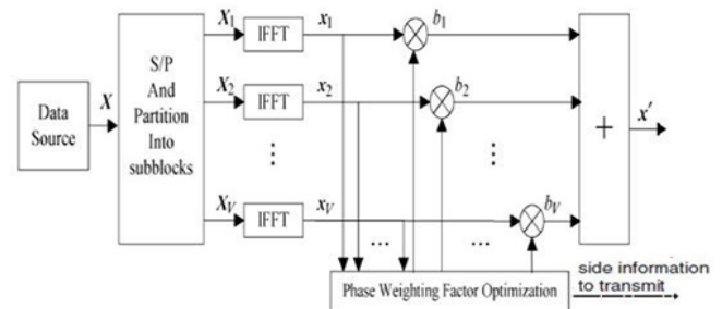
Figure 4. Block Diagram of PTS Technique
