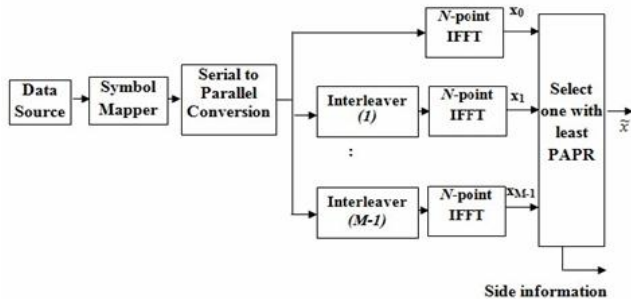
Figure 4. Interleaved OFDM Techniques
