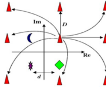
Figure 5. Extended Constellation in QPSK
