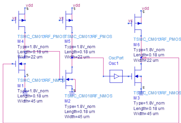
Figure 4. A typical Ring CURRENT CONTROLLED OSCILLATOR
