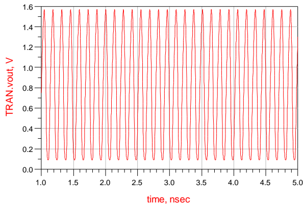
Figure 8. The simulation results of CURRENT CONTROLLED OSCILLATOR for Vc=0.5 V
