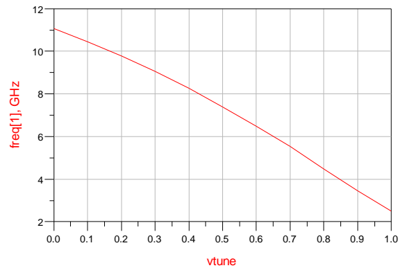
Figure 9. The oscillation frequency as a function of voltage control
