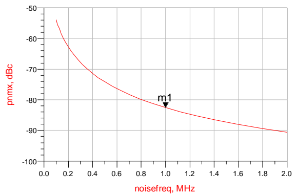
Figure 10. The phase noise of this oscillator for Vc=0.5 V
