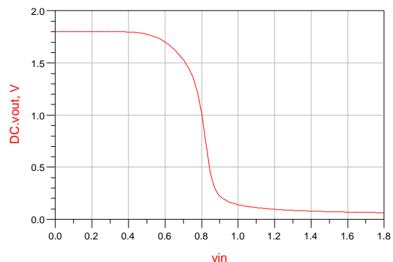
Figure 6 the drain voltage versus gate voltage
