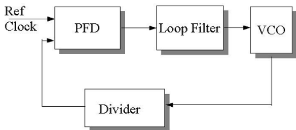
Figure1. A typical PLL circuit block diagram
