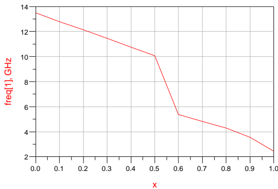
Figure 12 the frequency range of proposed oscillator.
