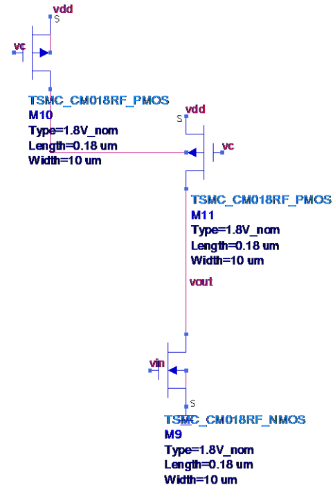
Figure 5 one stage of ring oscillator
