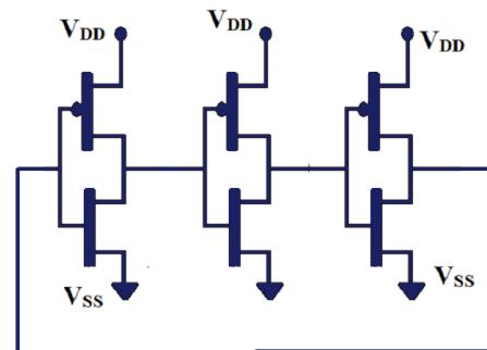
Figure 2 A ring oscillator consists of multiple delay cells
