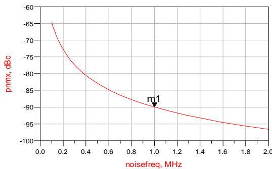
Figure 13 the phase noise of proposed oscillator
